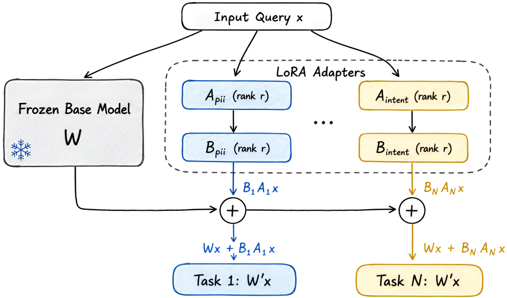
Figure 17 LoRA-based MoM inference architecture. The input query \mathbf{x} is processed by a single frozen base model ( W ). Each task-specific LoRA adapter pair ( A_i, B_i ) computes a low-rank perturbation B_i A_i \mathbf{x} . The base output and adapter perturbation are summed to produce task-specific classifications, enabling multi-task support with minimal memory overhead.
